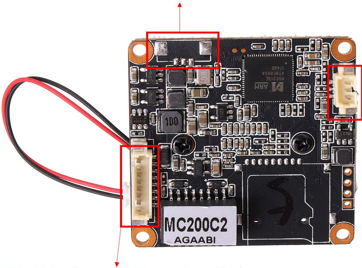
D1: 8pin Network & Power interface
