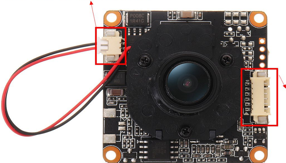
D4: 2pin IR-CUT interface
